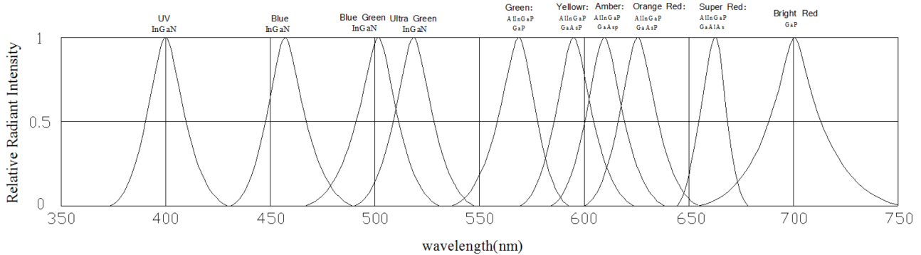
Relative Intensity VS. wavelength
